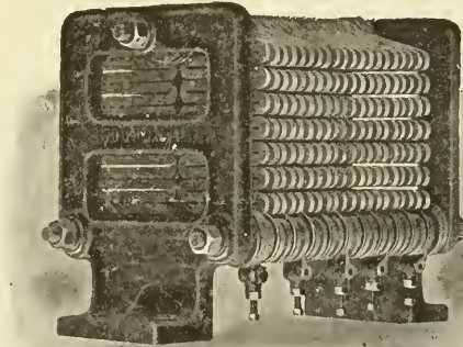
Fig. 121. Typical Rheostat with Cast-Iron Grids
